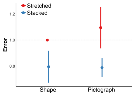
Fig. 5. Error levels are scaled relative to the error level of the simple bar chart, so it has 1.0 error for all subjects (top-left point). Charts with stacked items (blue) produced less error than those with stretched items (red). The use of simple shapes (left) or pictographs (right) had little impact.
